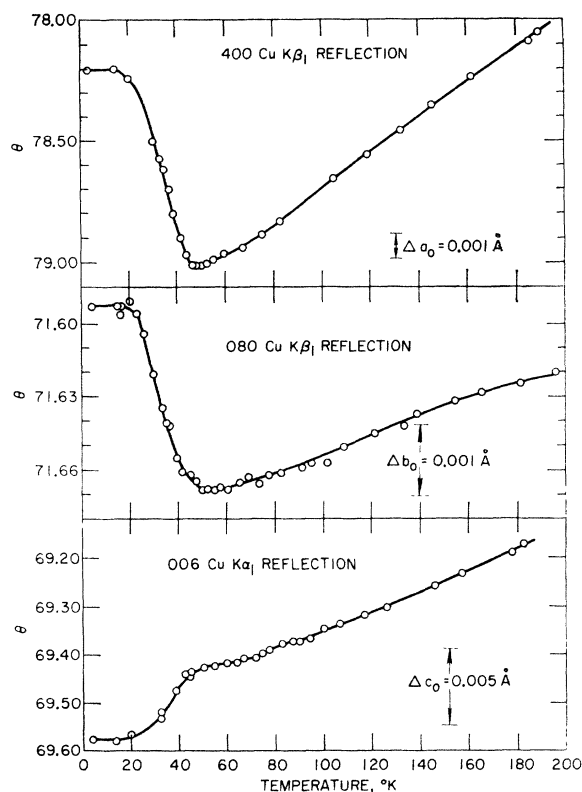
FIG. 1. Relative change of 400, 080, and 006 reflections for alpha uranium as a function of temperature. Angle \theta in degrees.
