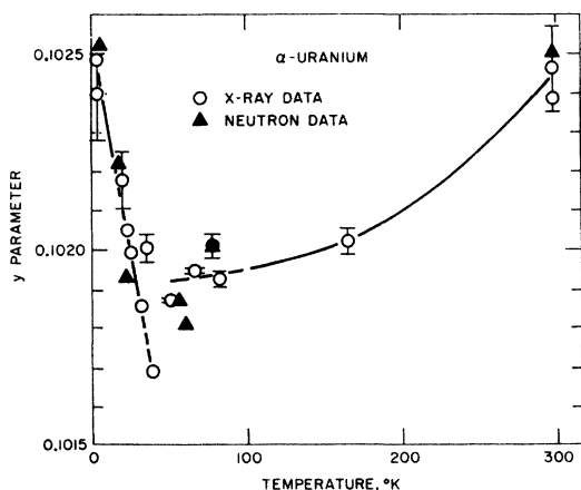
FIG. 3. The atomic position parameter, y , of alpha uranium as a function of temperature.
