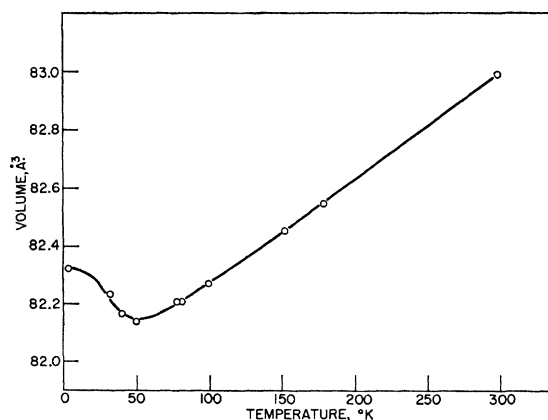
FIG. 2. Volume change for alpha uranium as determined from the lattice constants.
