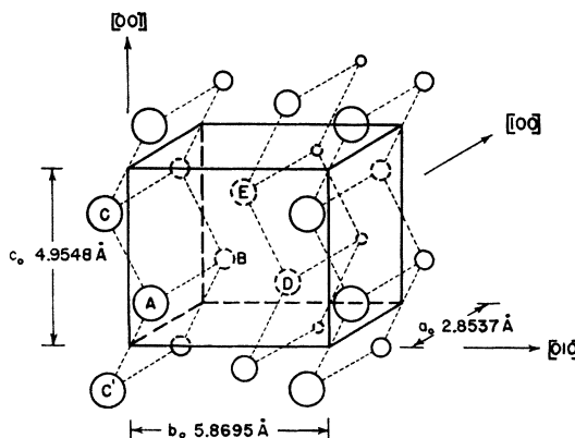
FIG. 4. Atomic arrangement in alpha uranium with room-temperature lattice constants.
